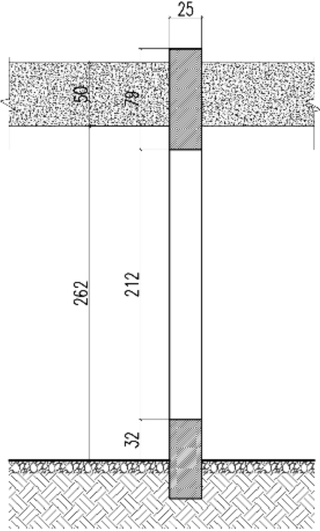
2 紫藤框牆剖面圖 W-09 Scale:1/40 cm
